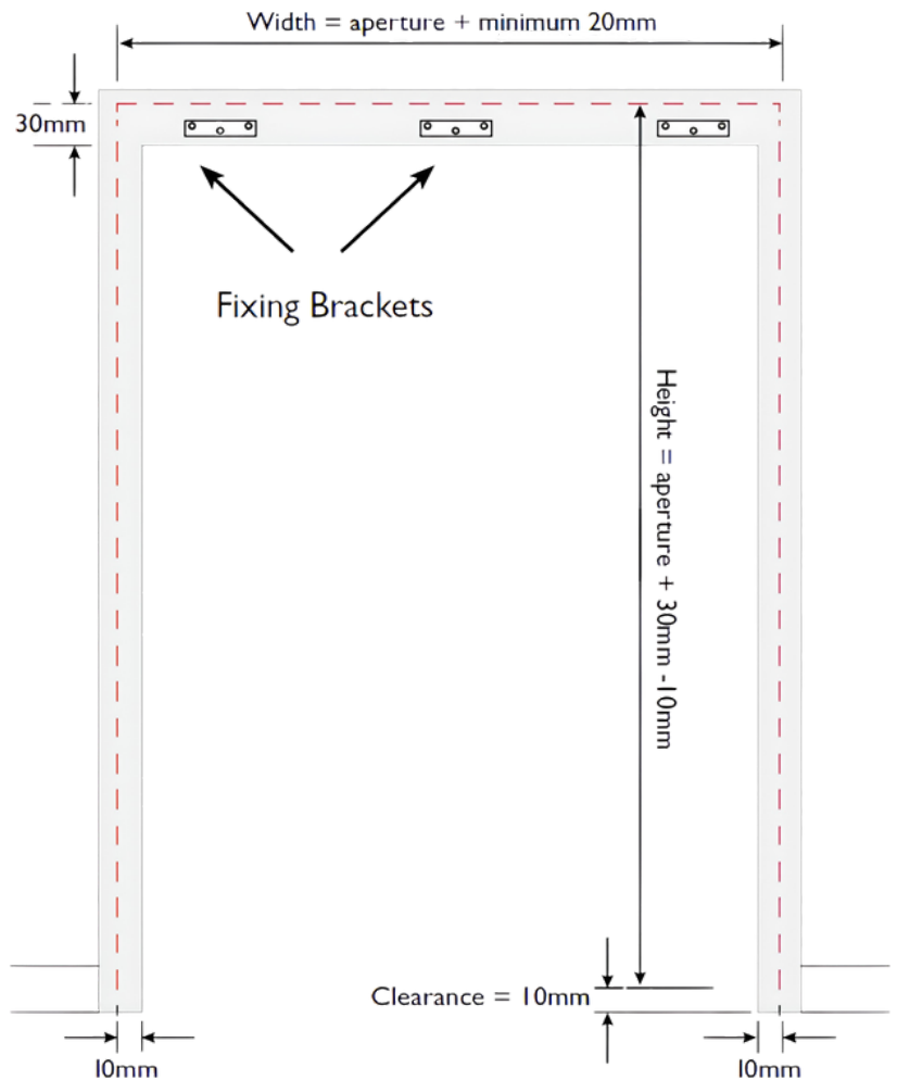
Stainless Steel Fixing Brackets
